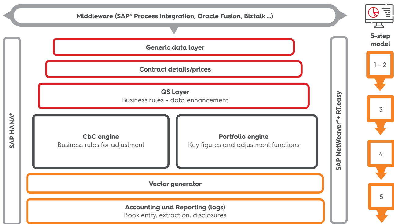
Fig. 2: IFRS15.easy architecture
